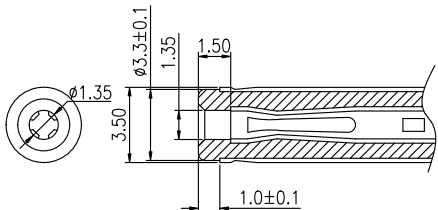
MATE PLUG
